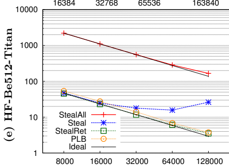
Figure 5: Execution times for first and last iteration. x-axis — number of cores; y-axis — execution time in seconds
