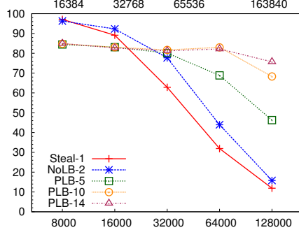
Figure 6: Efficiency of persistence-based load-balancing across iterations for the three system sizes, relative to the ideal anticipated speedup. x-axis — number of cores; y-axis — efficiency
