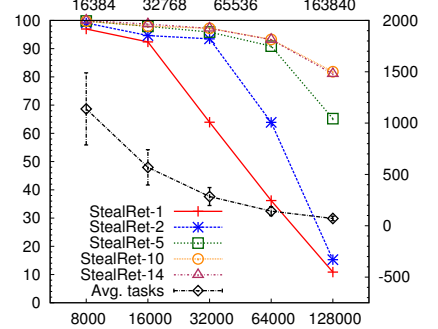
Figure 7: Efficiency of retentive work stealing across iterations relative to ideal anticipated speedup and tasks per core. x-axis — core count; left y-axis — efficiency; right y-axis — tasks per core (error bar: std. dev.)
