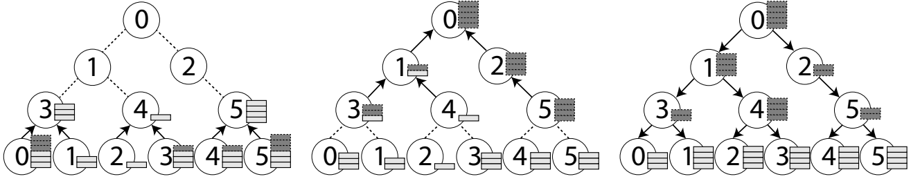
(a) All the leaves of the tree send their excess load (any load above a constant, referred to as C , times the average load) to their parent, selecting the work units from shortest duration to longest.
