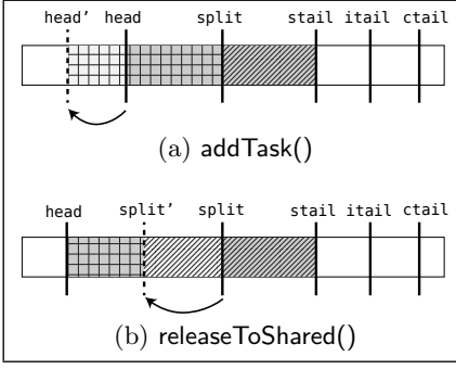
Figure 2: Routines related to adding tasks into the deque
